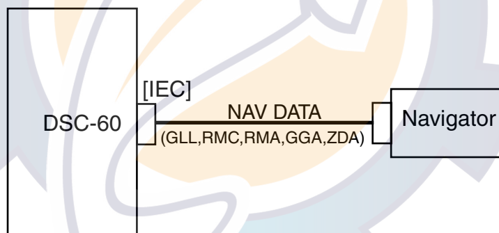
Navigator connection
